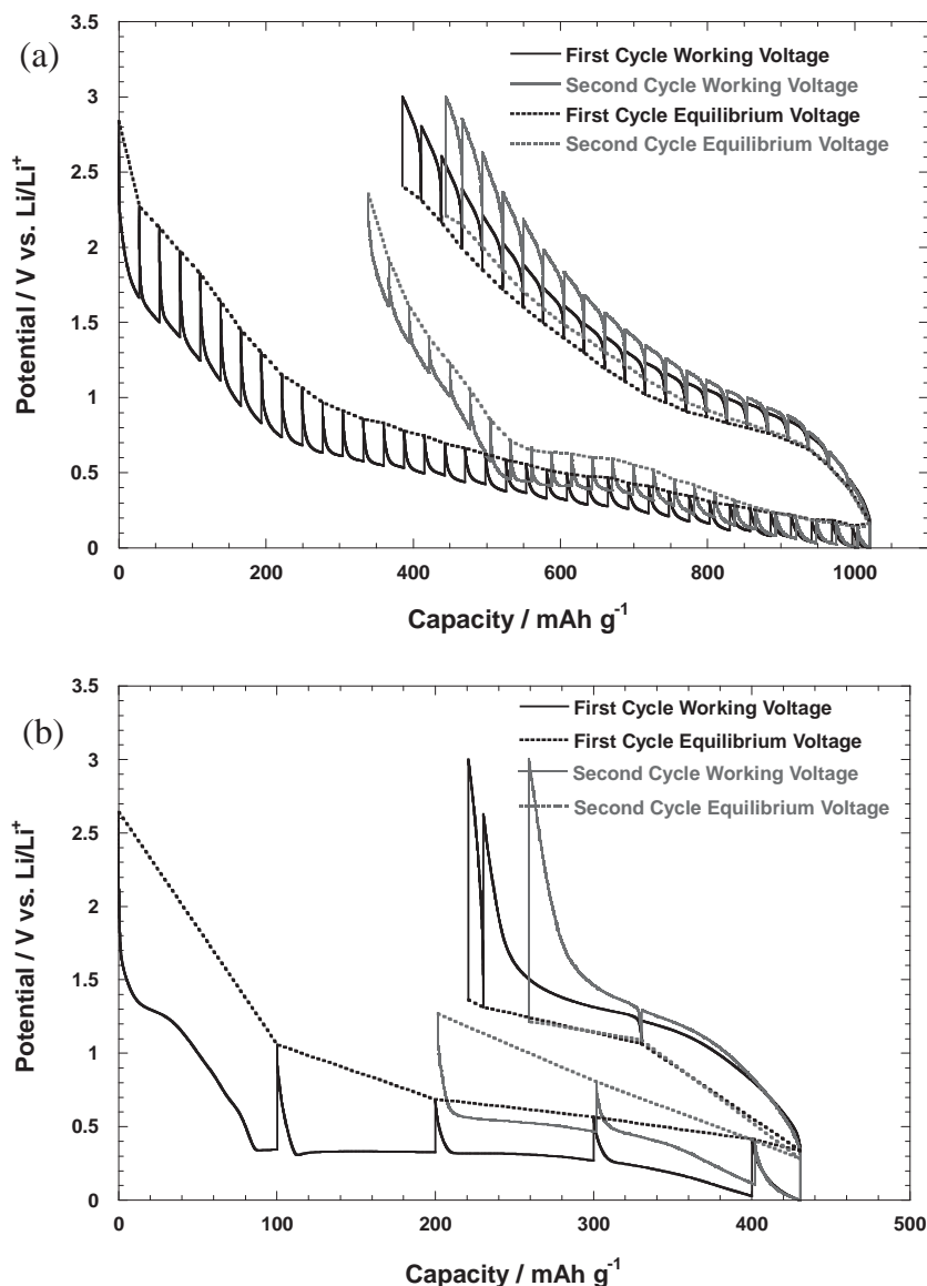
Figure 9. GITT curves of amorphous MnO x -C nanoparticles (a) and crystalline MnO x nanoparticles (b).
